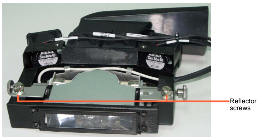
Figure 6-99: UV-reflector screws
