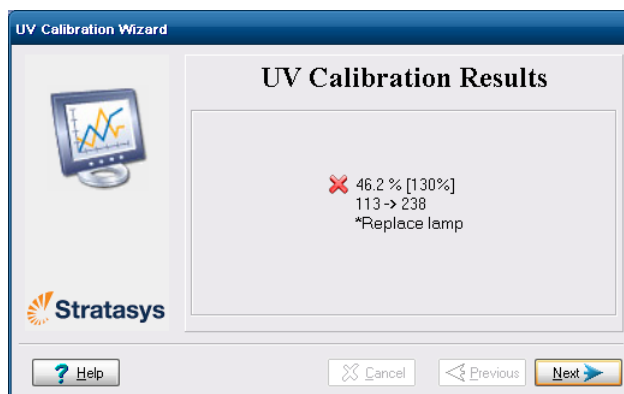
Figure 6-86: Final condition of UV lamp—unacceptable intensity level
