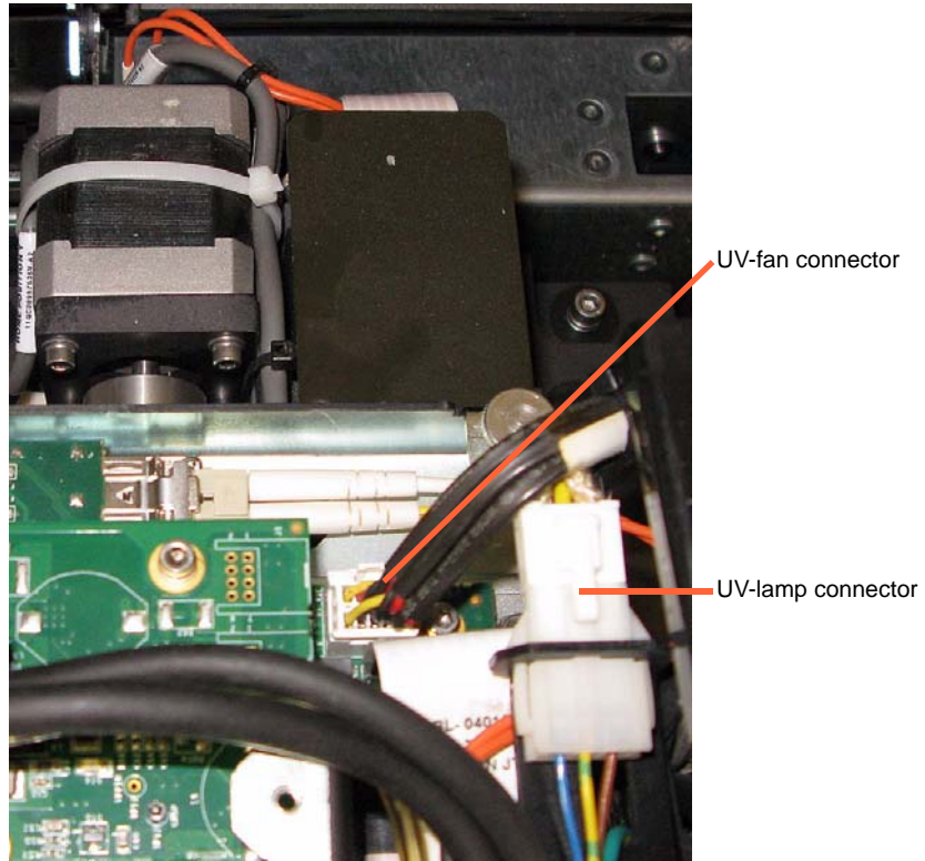
Figure 6-96: Disconnecting the UV lamp assembly (top view)
