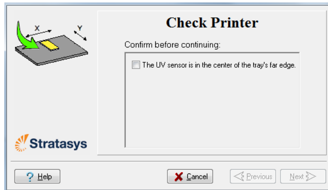
Figure 6-88 Sensor placement screen
