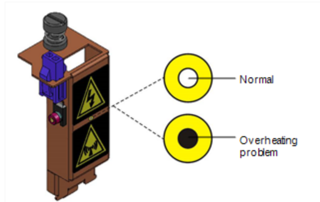
Figure 6-20 Heat-sensitive label on UV lamp cover
