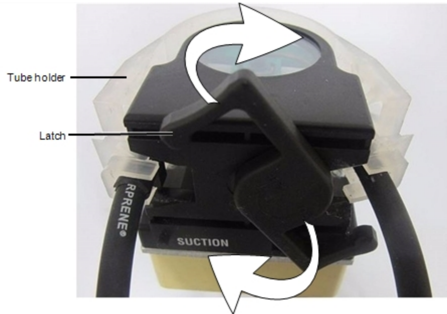
Figure 6-94 Releasing the tube latch
