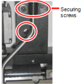
Figure 6-37 Suction tube correctly positioned
