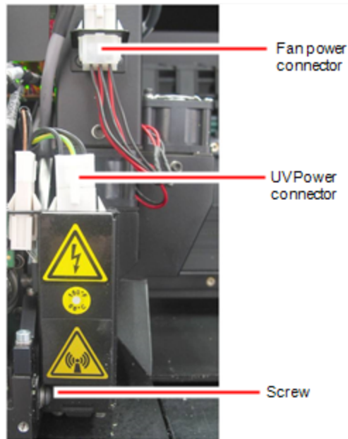
Figure 6-31 Disconnecting the right UV assembly
