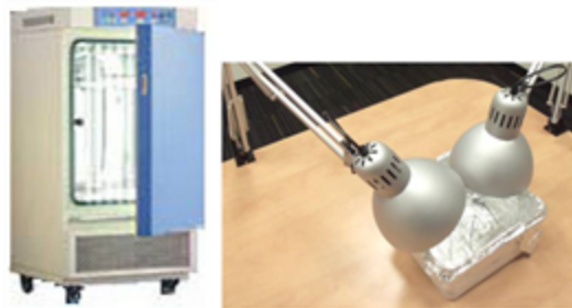
Figure 7-3 Left: Illumination chamber; Right: Desk lamps
