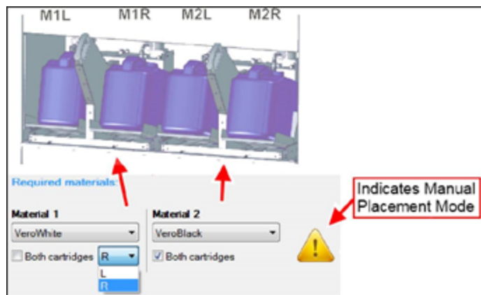
Figure 6-15 Manual cartridge placement
