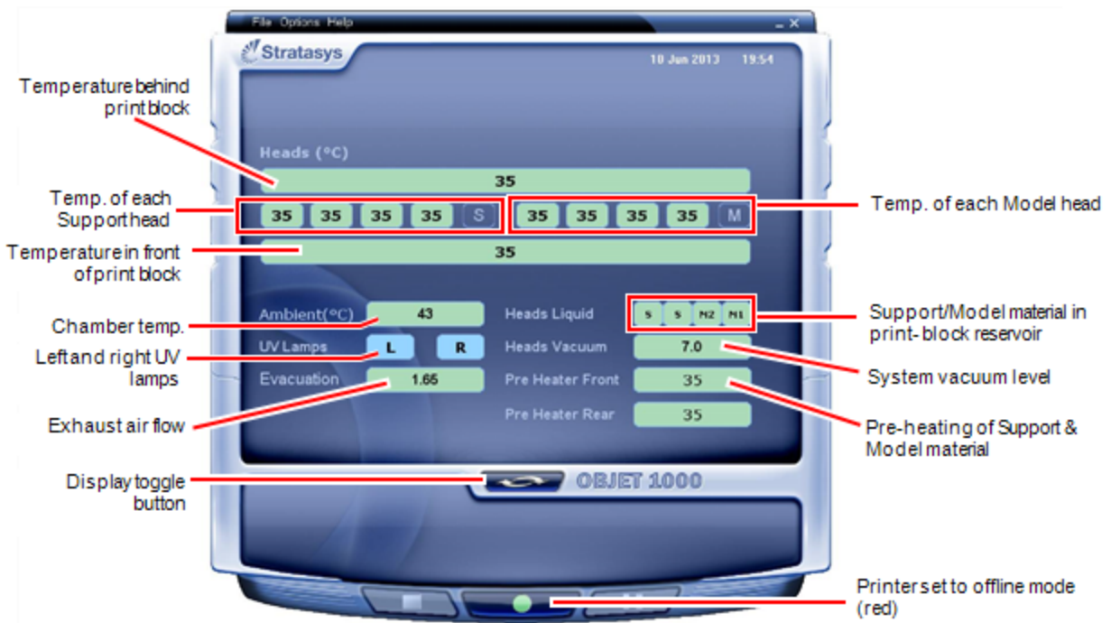
Figure 6-5 Printer status
