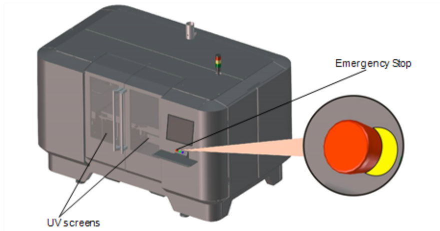
Figure 2-1 Objet1000 Plus—front view
