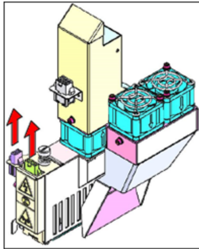
Figure 6-105 Disconnecting the UV lamp
