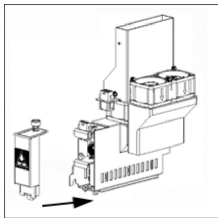
Figure 6-109 Replacing the UV lamp cover
