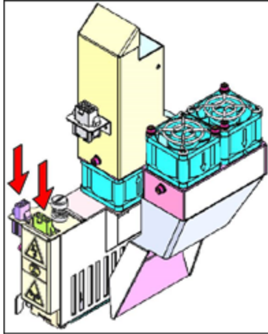
Figure 6-110 Connecting the UV lamp
