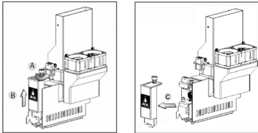
Figure 6-106 Removing the UV lamp cover
