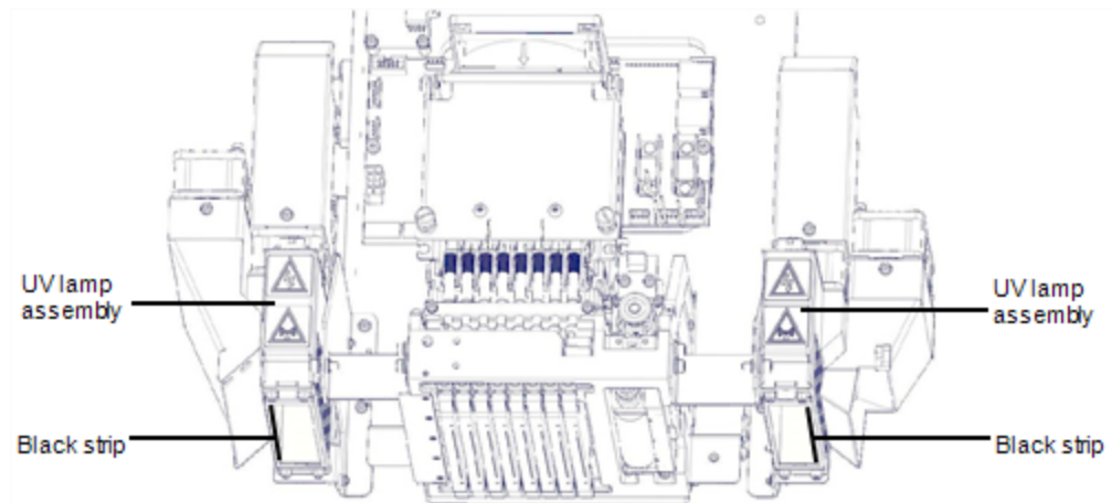
Figure 6-108 Print block and UV lamp assembly, showing correct placement of black strip
